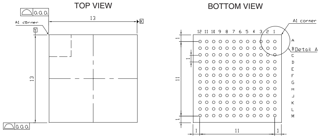
Figure 5. 144-ball BGA Package Drawing
